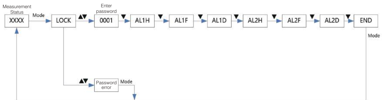
Figure 5-5 Switch point setting flow chart
