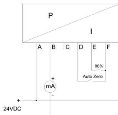
4...20mA Output (2-wire)
