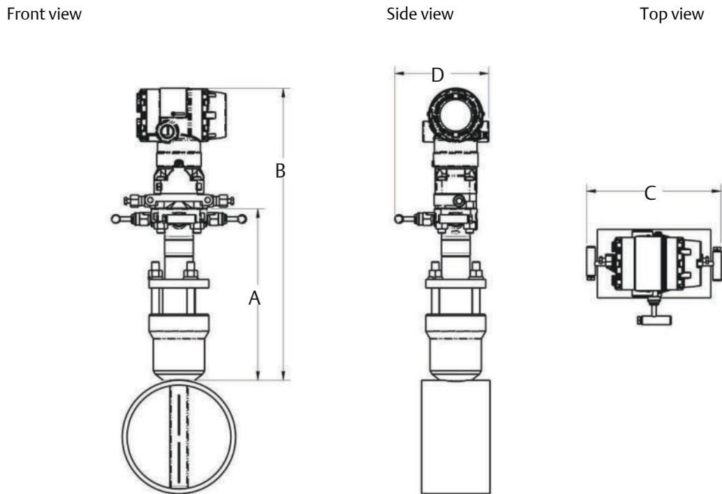
Figure 25: Rosemount 2051CFA Annubar Pak-Lok Flow Meter
