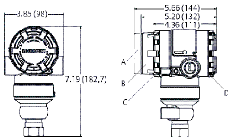
Figure 16: Rosemount 2051T
